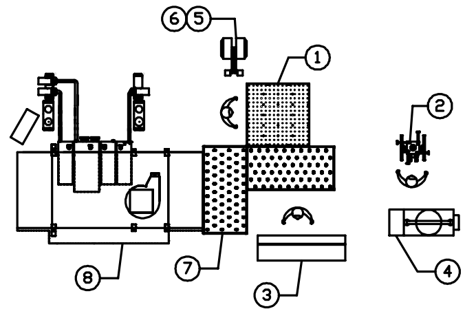
SWIFT SHOP LAYOUT V/ OPTIONAL UPGRADED AIRFLOAT TABLE 60X60 ■ PRODUCTION 150 UNITS PER 8 HOUR SHIFT
